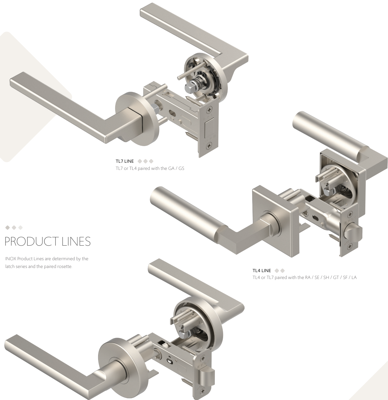
TL3 LINE ◆◆◆ TL3 Latch paired with the RA / SE
