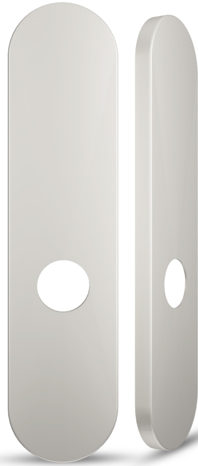
LA SERIES 10-1/2" x 2-1/2" x 7/16" Plate (267 mm X 63 mm x 11 mm)
