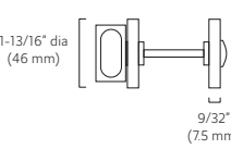
GR PRIVACY SET Passage w/ Privacy Bolt
