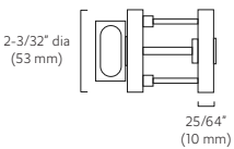
GT PRIVACY SET Passage w/ Privacy Bolt
