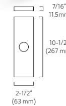
SF SERIES 10-1/2" x 2-1/2" x 7/16" Plate (267mm x 63 mm x 11 mm)
