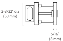
GS PRIVACY SET Passage w/ Privacy Bolt
