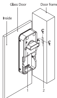
For Right Handed Glass Door
