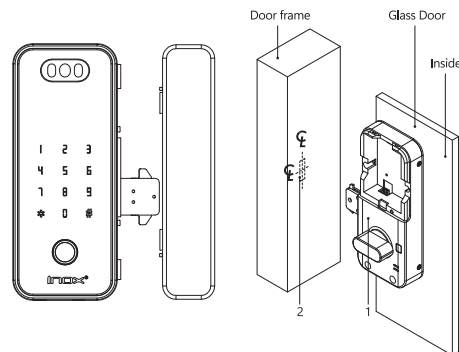
For Left Handed Glass Door
