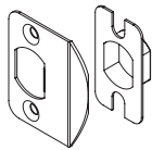
Full-lip Strike 1/4" Corner LSR-D14 1-3/4" x 2-1/4"
