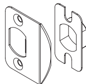
Full-lip Strike 1/4" Corner LSR-D14 1-3/4"x2-1/4"
